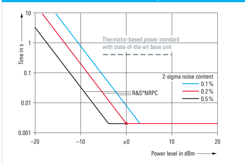
Achievable measurement times per frequency point for the R&S®NRPC and for a thermistor-based power standard
