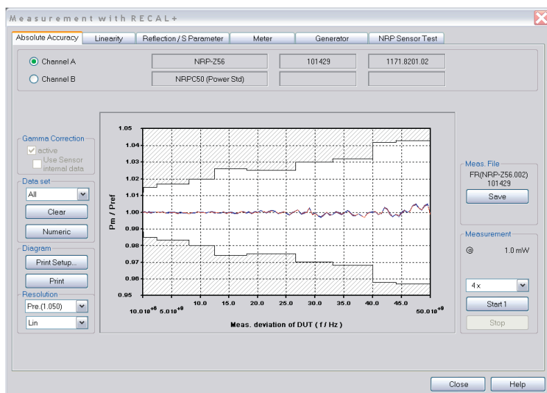
User interface of the R&S®Recal+ PC software with graphical display of the calibration result for an R&S®NRP-Z56 50 GHz thermal power sensor.
